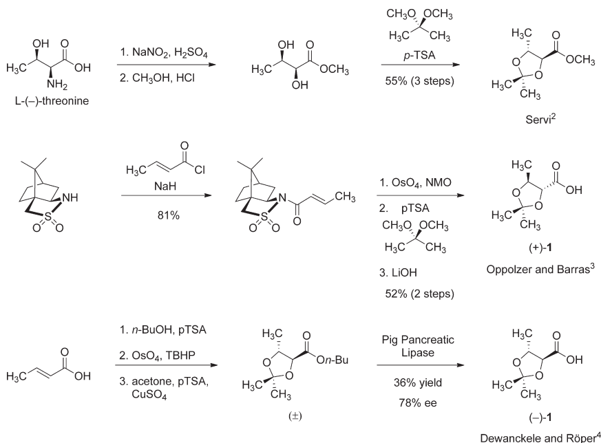
Scheme 1. Prior Syntheses of syn -2,3-Dihydroxybutyrate and Its Methyl Ester
