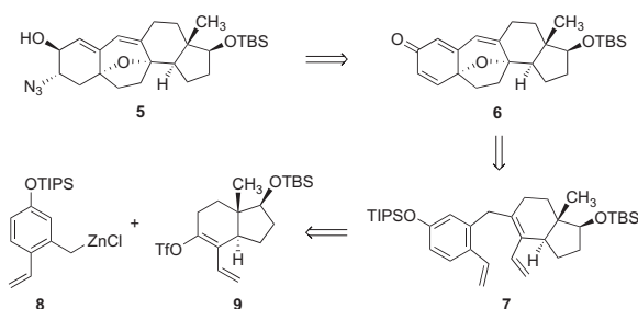
Figure 2 | A key precursor to cortistatins and its retrosynthetic disconnection. The azido alcohol intermediate 5 serves as a common intermediate for the synthesis of cortistatins A, J, K and L, as well as cortistatin analogues. This intermediate arises in turn from the cyclohexadienone 6 and the triene 7 . The latter intermediate is formed by coupling of the o -vinyl benzylzinc reagent 8 and the enol triflate intermediate 9 . TBS, tert -butyldimethylsilyl; TIPS, triisopropylsilyl; Tf, trifluoromethanesulfonyl.
