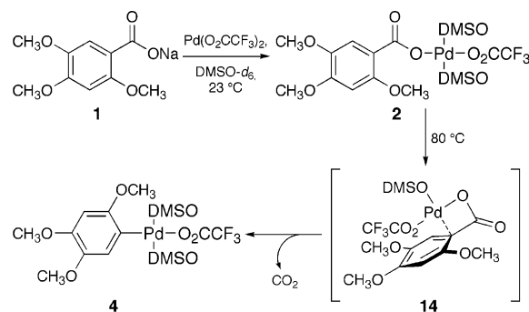
Scheme 3. Proposed Mechanism of Decarboxylative Palladation
