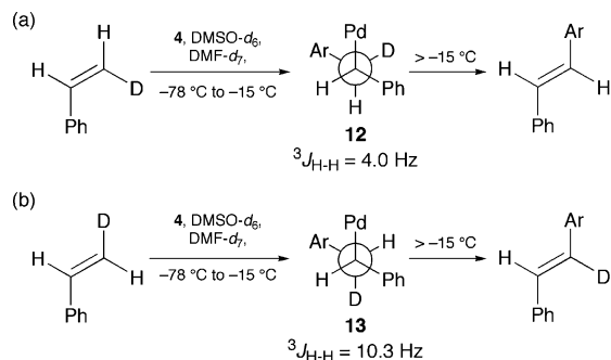
Scheme 2. ^1\text{H} NMR Studies Establishing the Stereochemical Course of the Olefin Insertion and \beta -Hydride Elimination Reactions of the \beta -D-Styrene Derivatives (a) cis - \beta -D-Styrene and (b) trans - \beta -D-Styrene a
