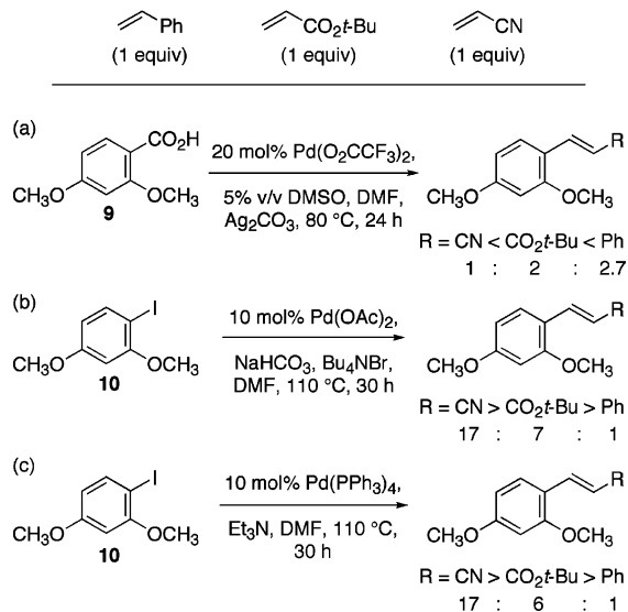
Scheme 1. Summary of Competitive Olefination Experiments with Styrene, tert -Butyl Acrylate and Acrylonitrile (1 equiv each) a
