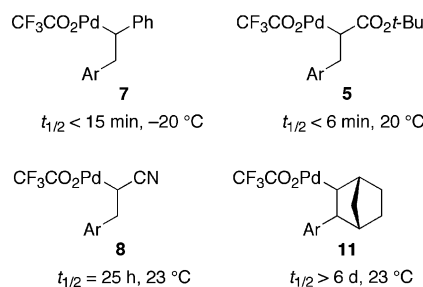
Figure 5. Half-lives of observed \sigma -aryl palladium(II) intermediates 5 , 7 , 8 , and 11 . In each case, the \sigma -aryl palladium(II) intermediate was transformed cleanly into the corresponding Heck-type product. Thus, the half-lives provide an estimation of the rate of \beta -hydride elimination in each case.
