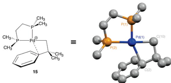
Figure 8. Structure of a \sigma -aryl palladium(II) intermediate 15 showing a \pi , \eta^1 palladium–arene interaction. 17 The counterion is tetrakis[3,5-bis-(trifluoromethyl)phenyl]borate (BARF) and has been omitted for clarity. Selected bond lengths (Å) and bond angles (deg): Pd(1)–P(1) 2.220(2), Pd(1)–P(2) 2.363(2), Pd(1)–C(10) 2.065(7), Pd(1)–C(2) 2.343(6); P(1)–Pd(1)–P(2) 86.67(7), C(2)–Pd(1)–C(10) 66.2(3).
