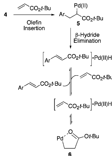
Scheme 5. Plausible Sequence for the Formation of the Palladacycle 6 from the \sigma -Arylalkylpalladium(II) Intermediate 5 (see ref 8)
