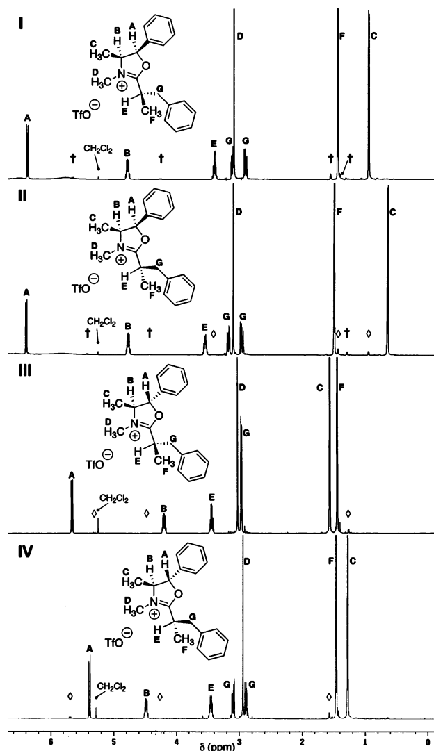
Figure 1. \delta -0.2 – 6.7 ppm region of ^1\text{H} NMR spectra of the cyclization products of Scheme 1 ( \text{CDCl}_3 , 23^\circ\text{C} ). Spectra are referenced to residual protium in the NMR solvent ( \text{CHCl}_3 , \delta 7.26).
