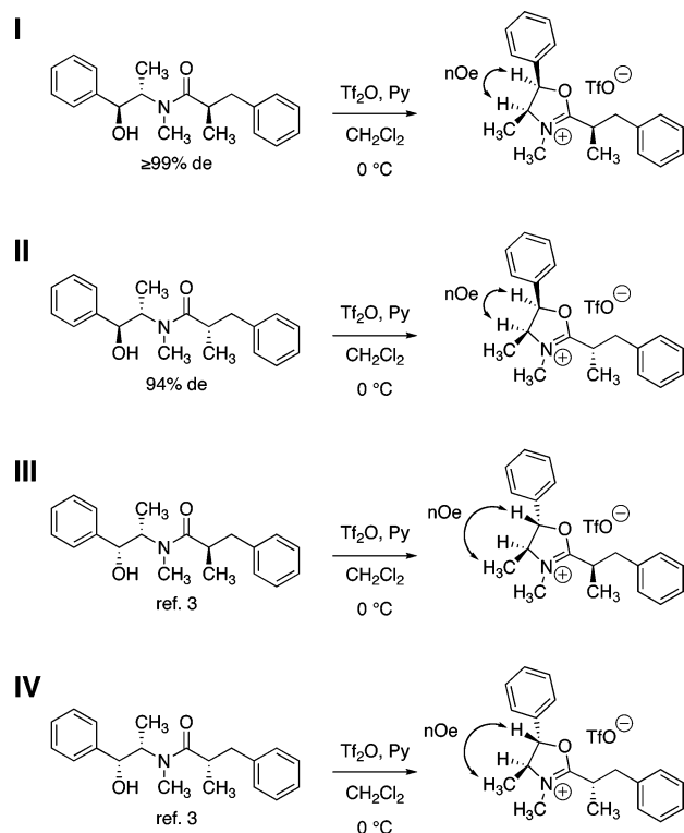
Scheme 1. Reaction of Pseudoephedrine (I and II) and Ephedrine (III and IV) Amides of (+)- and (–)- \alpha -Methylbenzenepropanoic Acid with Triflic Anhydride–Pyridine To Form 4,5-Dihydro-3,4-dimethyl-5-phenyl-1,3-oxazolium Triflate Derivatives
