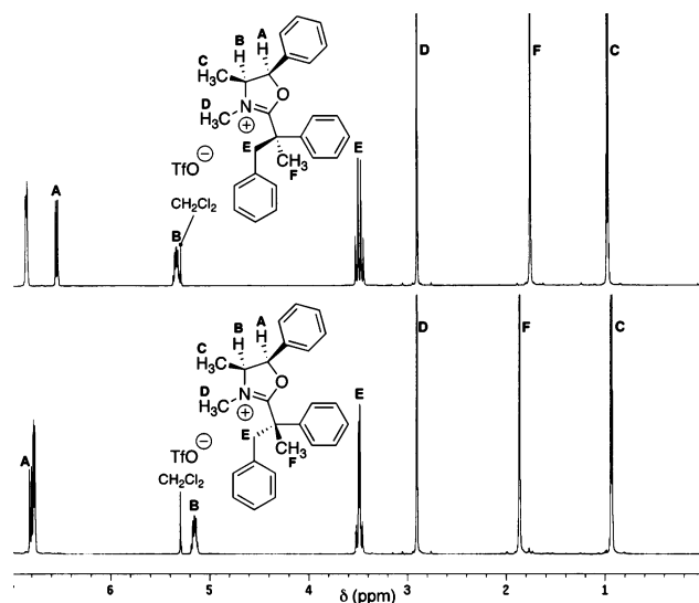
Figure 2. \delta 0–7.0 ppm region of ^1\text{H} NMR spectra of the cyclization products ( \text{CDCl}_3 , 23 ^\circ\text{C} ). Spectra are referenced to residual protium in the NMR solvent ( \text{CHCl}_3 , \delta 7.26).
