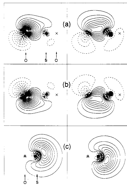
Figure 1. GVB orbitals for SO 2 using a DZ+d(O,S) basis set. (a, b) Orbitals representing the S=O double bond. (c) Angularly correlated S lone pair. Contours are separated by 0.04 au in both figures.
