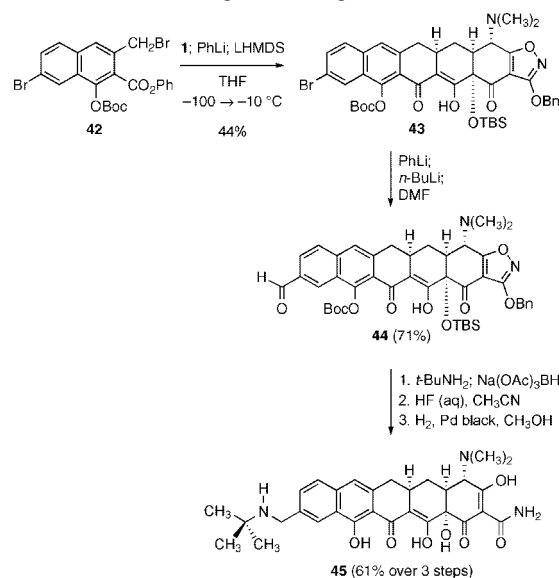
Scheme 14. Synthesis of the Diversifiable Pentacycline Precursors 43 and 44 by Michael–Claisen Cyclization Using the Benzylic Bromide 42 and Enone 1 as Substrates, with an in Situ Protocol for Selective Lithium–Halogen Exchange a
