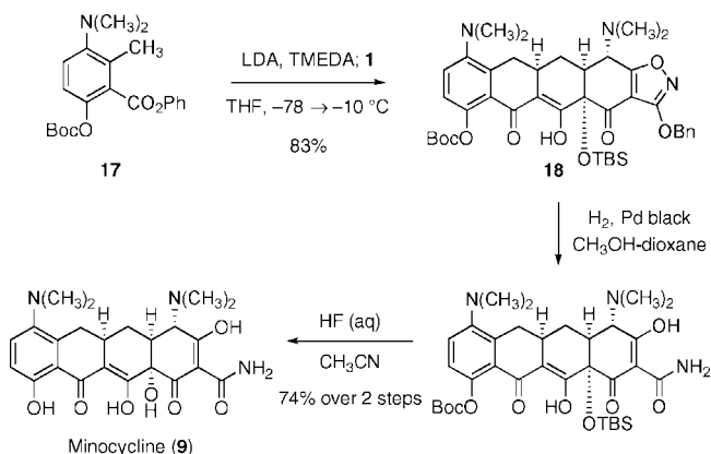
Scheme 3. Synthesis of Minocycline ( 9 ) by Michael–Claisen Cyclization Using the tert -Butoxycarbonyl-Protected Phenyl Ester 17 as the D-Ring Precursor and a Stepwise Protocol for Addition of the Base and Enone 1 , Followed by Deprotection
