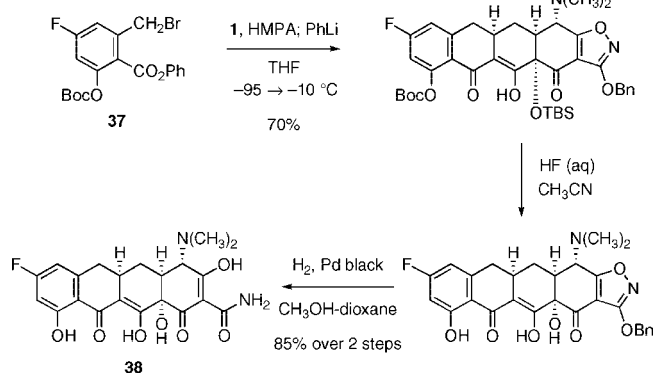
Scheme 11. Synthesis of 10-Deoxysancycline ( 41 ) by Michael–Claisen Cyclization Using Phenyl 2-(Bromomethyl)benzoate ( 39 ) and Enone 1 as Substrates, with Deprotonation in Situ, Followed by Deprotection
