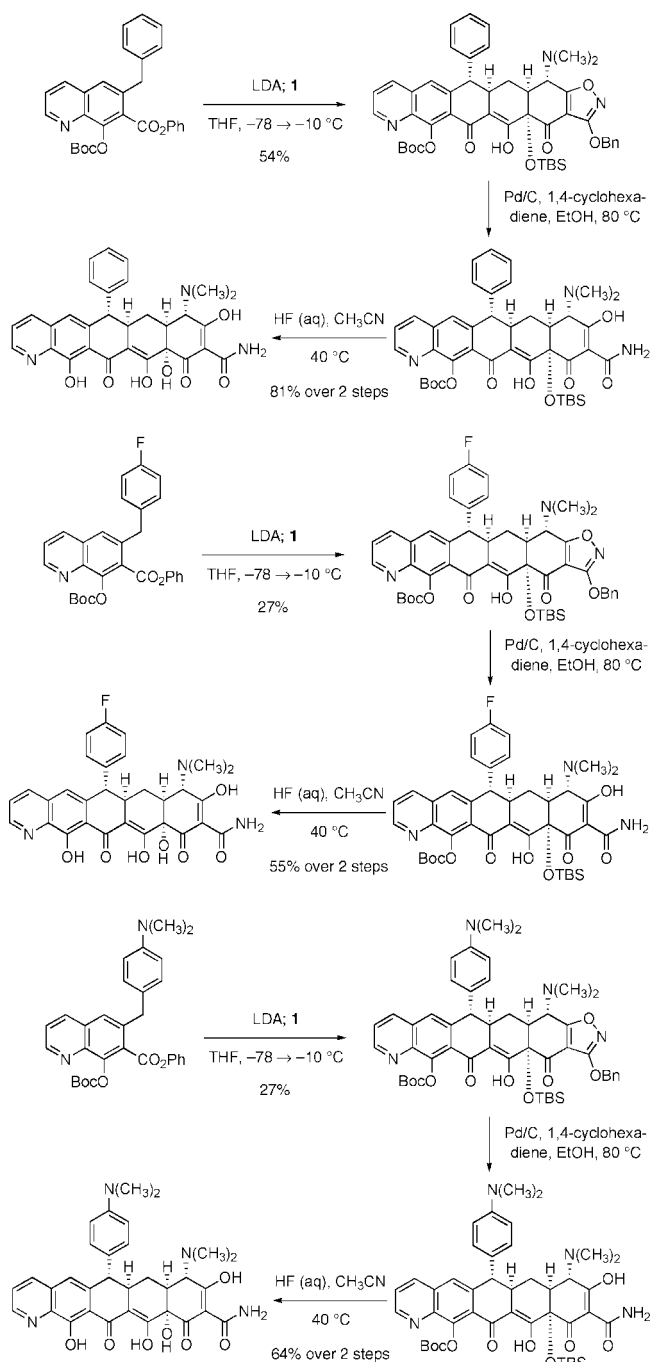
Scheme 13. Synthesis of 6-Aryl-Substituted Heterocyclic Pentacyclines by Michael–Claisen Cyclizations Using Benzylically Substituted Quinolines as DE-Ring Precursors and a Stepwise Protocol for Addition of the Base and Enone 1 , Followed by Deprotection
