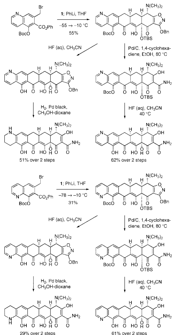
Scheme 12. Synthesis of Pentacyclines with Heterocyclic E Rings by Michael–Claisen Cyclizations Using Bromomethylquinolines and Enone 1 as Substrates, and an in Situ Protocol for Lithium–Halogen Exchange, Followed by Deprotection
