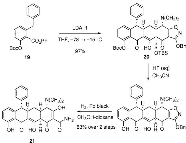
Scheme 4. Synthesis of 6-( S )-Phenylsancycline ( 21 ) by Michael–Claisen Cyclization Using the tert -Butoxycarbonyl-Protected Phenyl Ester 19 as the D-Ring Precursor and a Stepwise Protocol for Addition of the Base and Enone 1 , Followed by Deprotection
