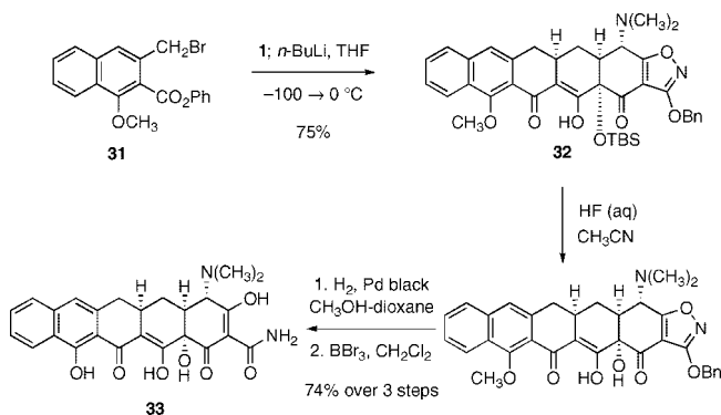
Scheme 8. Synthesis of the Pentacycline 33 by Michael–Claisen Cyclization Using the Phenyl Bromomethylnaphthoic Acid Ester 31 and Enone 1 as Substrates, and an In Situ Protocol for Lithium–Halogen Exchange, Followed by Deprotection
