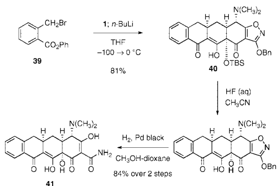
Scheme 11. Synthesis of 10-Deoxysancycline ( 41 ) by Michael–Claisen Cyclization Using Phenyl 2-(Bromomethyl)benzoate ( 39 ) and Enone 1 as Substrates, with Deprotonation in Situ, Followed by Deprotection
