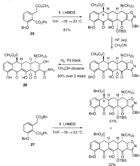
Scheme 6. Synthesis of 6-( S )-Carbomethoxysancycline ( 26 ) by Michael–Claisen Cyclization Using the Methyl Phenyl Diester 25 and Enone 1 as Substrates, with Deprotonation in Situ, Followed by Deprotection a
