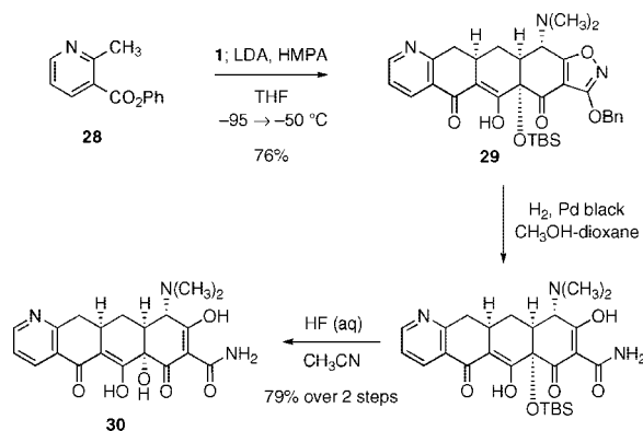
Scheme 7. Synthesis of 7-Aza-10-deoxysancycline ( 30 ) by Michael–Claisen Cyclization Using Phenyl Ester 28 and Enone 1 as Substrates, with Deprotonation in Situ, Followed by Deprotection
