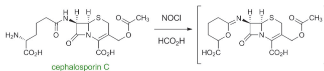
Scheme 4. Semisynthesis of 7-aminocephalosporanic acid (7-ACA) from cephalosporin C.
