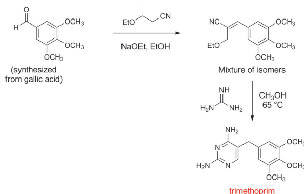
Scheme 8. Chemical synthesis of chloramphenicol and trimethoprim.
