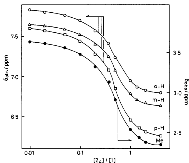
Figure 1. Plots of \delta_{\text{obs}} versus [2_4]/[1] . The concentration of 2 was maintained constant (1.00 mM) while that of 1 was varied (0.25–100 mM): D 2 O, 25 °C, pD 7.3 with 0.1 M phosphate buffer, internal standard DSS.
